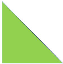
Right triangle
