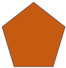
Pentagon
