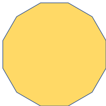
Dodecagon
