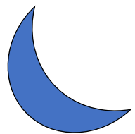
Crescent
