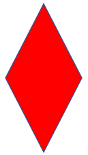
Diamond
