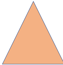
Isosceles triangle
