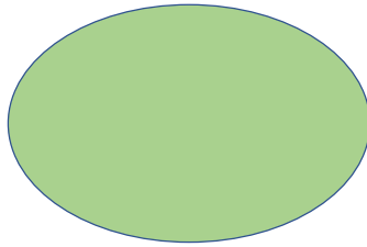
oval
