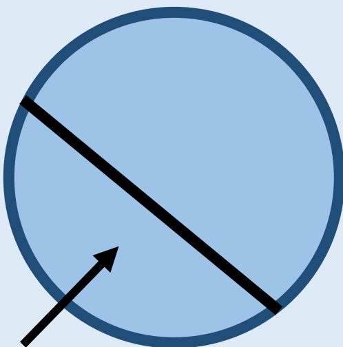
Chord
