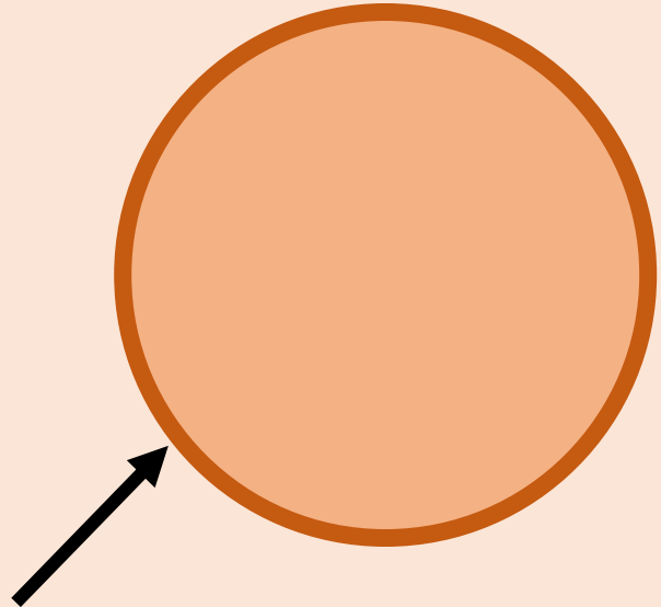
Circumference
