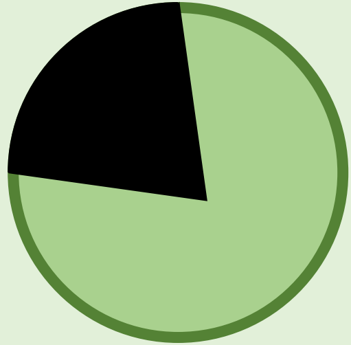
Sector
