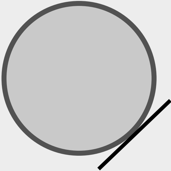
Tangent
