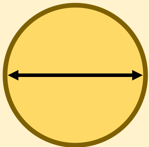
Diameter
