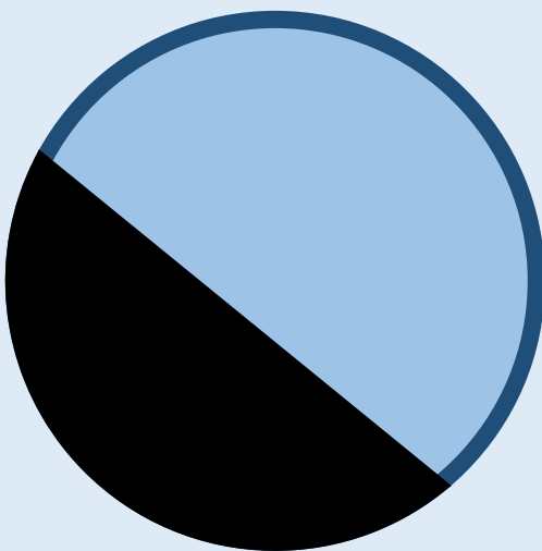
Segment
